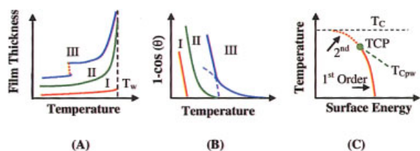
Figure 12. (A) For a solid in contact with a saturated vapor (that is, at vapor–liquid coexistence), a thin liquid film is formed at the solid surface and its thickness diverges smoothly or discontinuously as the temperature approaches the wetting point ( T_w ); (B) variation of the contact angle \theta near the wetting temperature: (I, II, and III stand for first-order, second-order, and sequence of wetting transitions, respectively); (C) when the fluid–solid interaction is short range, the first-order and the second-order wetting-transition lines join at the tricritical point (TCP) where the prewetting critical temperature ( T_{Cpw} ) terminates.
