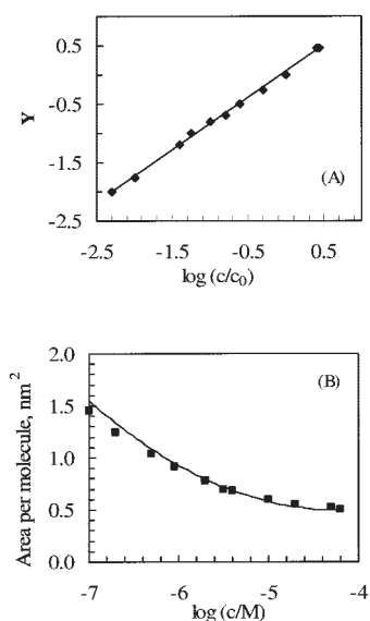
Figure 7. (A) A new scaling relation between the surface pressure ( \Pi ) and the bulk concentration of n -dodecyl pentaerythritol ether (C12E5) at the air–water interface; (B) surface area per C12E5 molecule vs. bulk concentration of the surfactant from SANS/ellipsometry measurements (points) and from DFT (lines) (reproduced from Stoyanov et al. 124 ).
